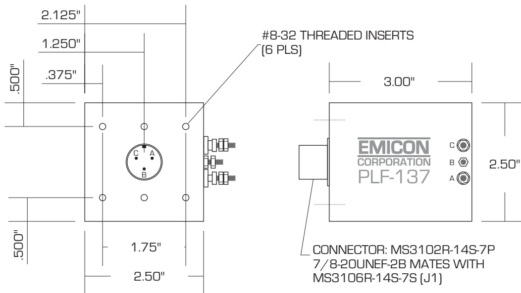
OUTLINE DRAWING
